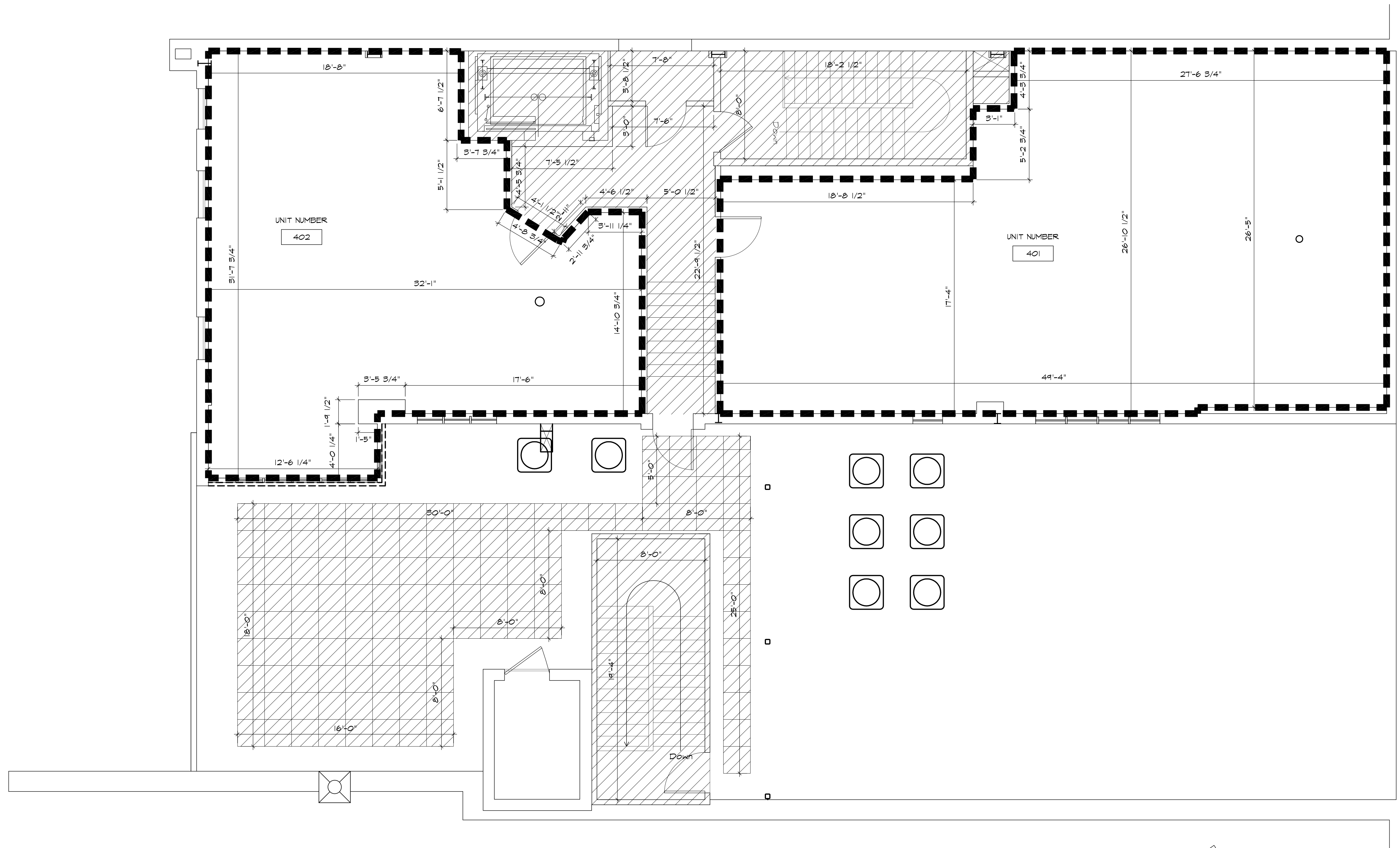
1 FOURTH FLOOR PLAN A1.4
